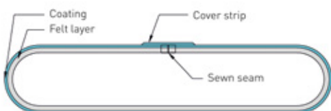
NORDIWALL Flex Lite is a coated needed felt hose
