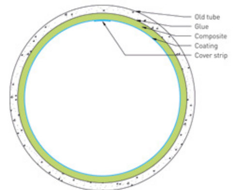
NORDIWALL Flex Lite seals joints and cracks and provides a structural pipe improvement
